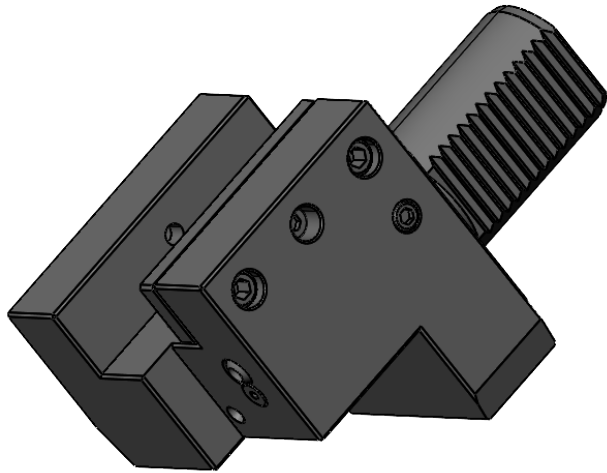
STRAIGHT VDI40 STATIC TOOL OUTPUT: 25mm SQR SHANK COOLANT: EXTERNAL
